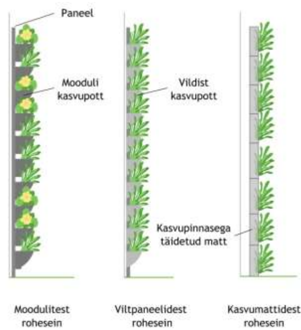
“Green/living wall”
